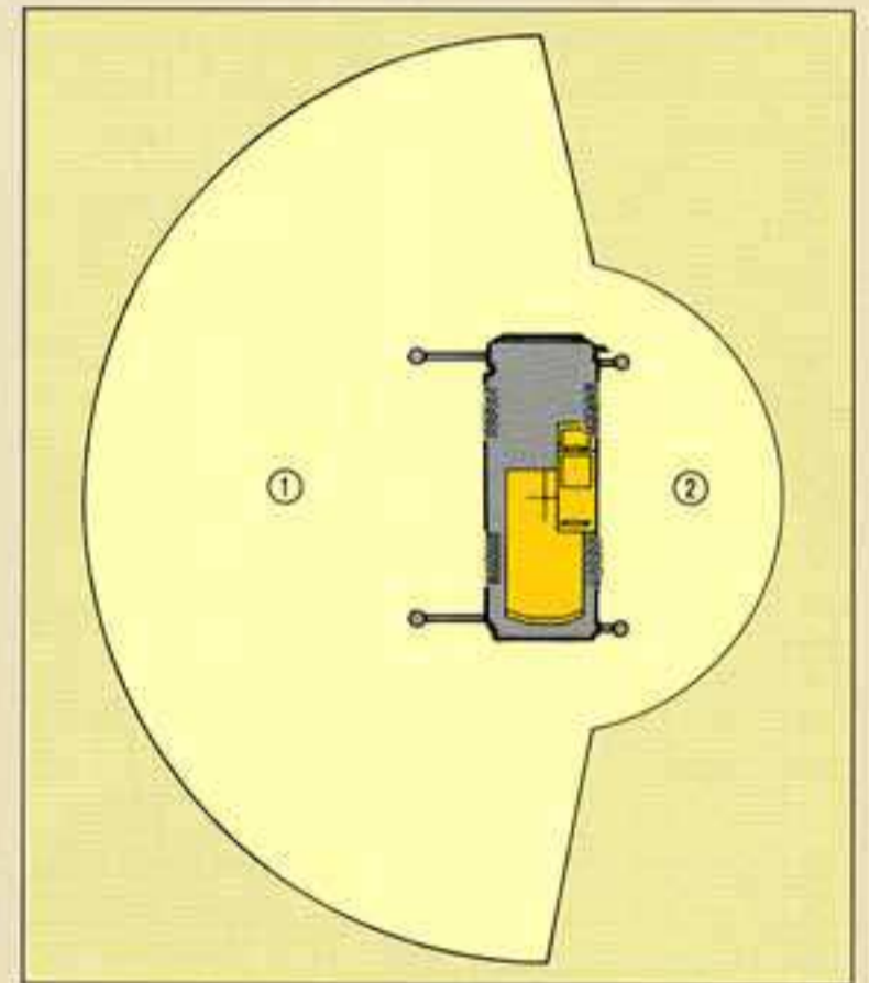
① Working range at maximum stroke ② Working range at intermittent stroke
